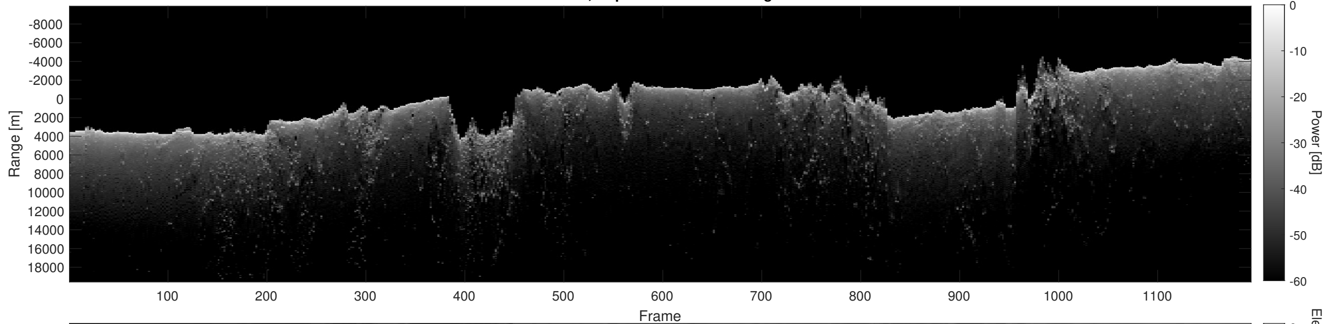
Orbit 4975, Depth-Corrected Cluttergram
