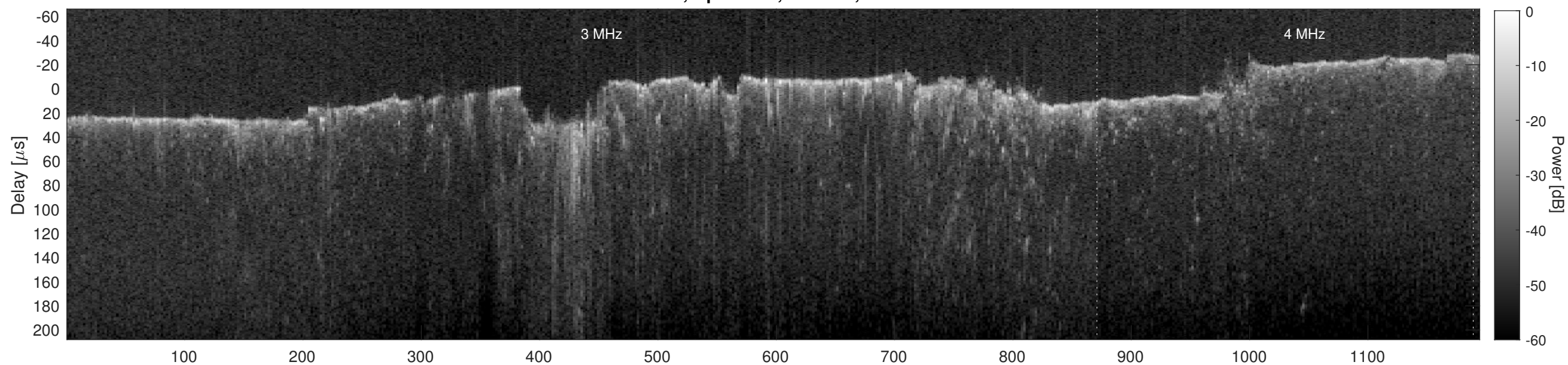
Orbit 4975, Cluttergram
