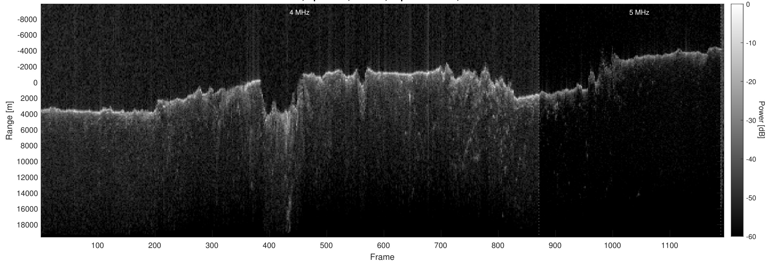
Orbit 4975, Optimized, Window, Depth-Corrected, Channel 2
