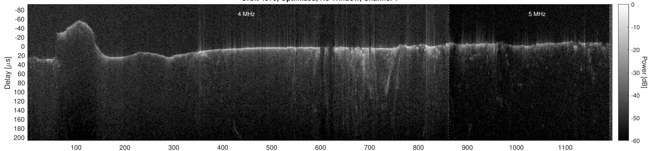
Orbit 4976, Optimized, No Window, Channel 2
