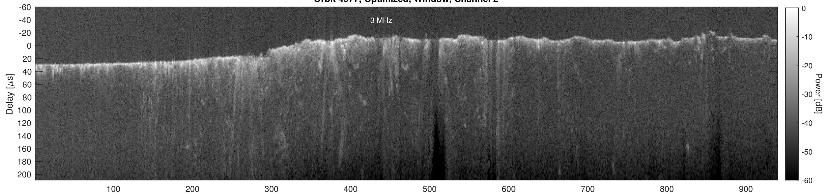
Orbit 4977, Cluttergram
