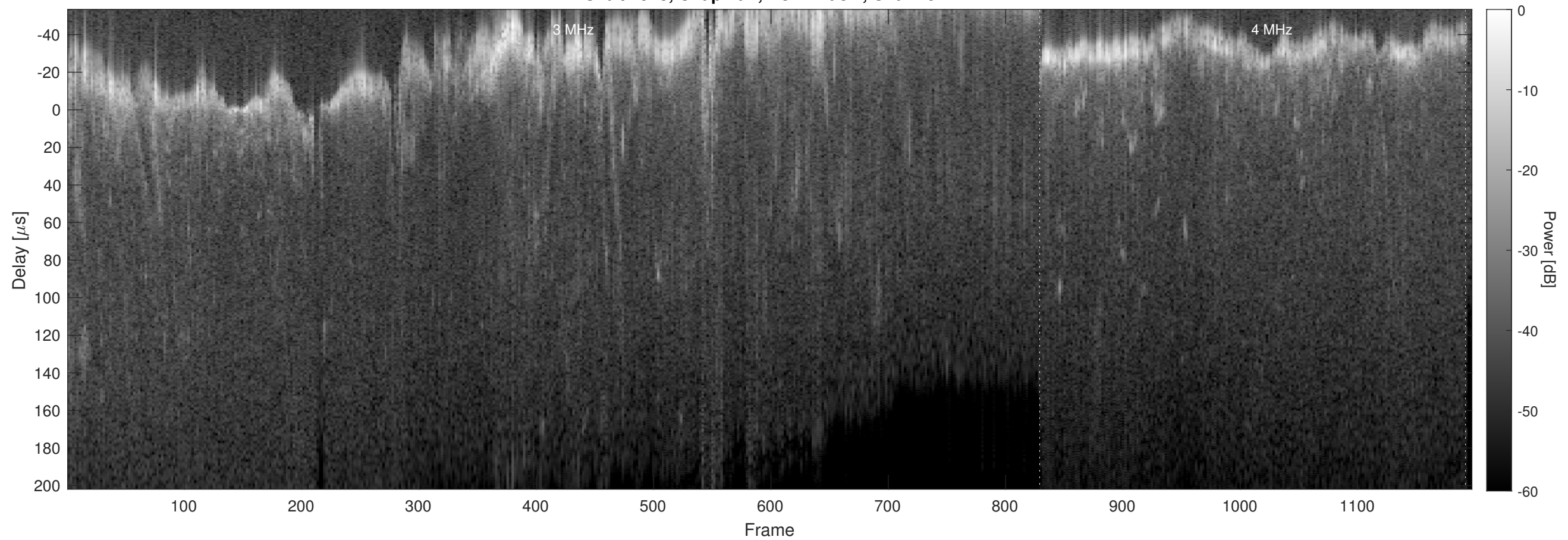
Orbit 4978, Chapman, No Window, Channel 2
