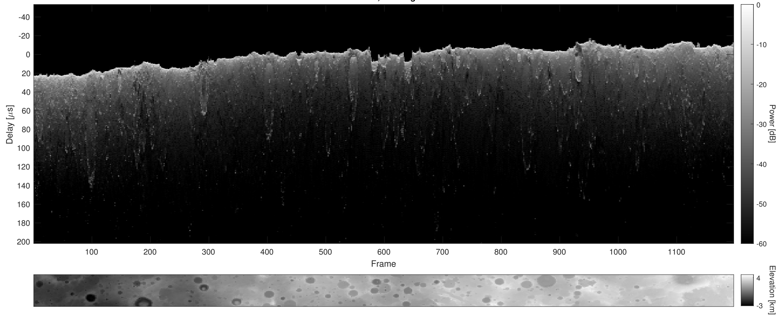
Orbit 4978, Cluttergram
