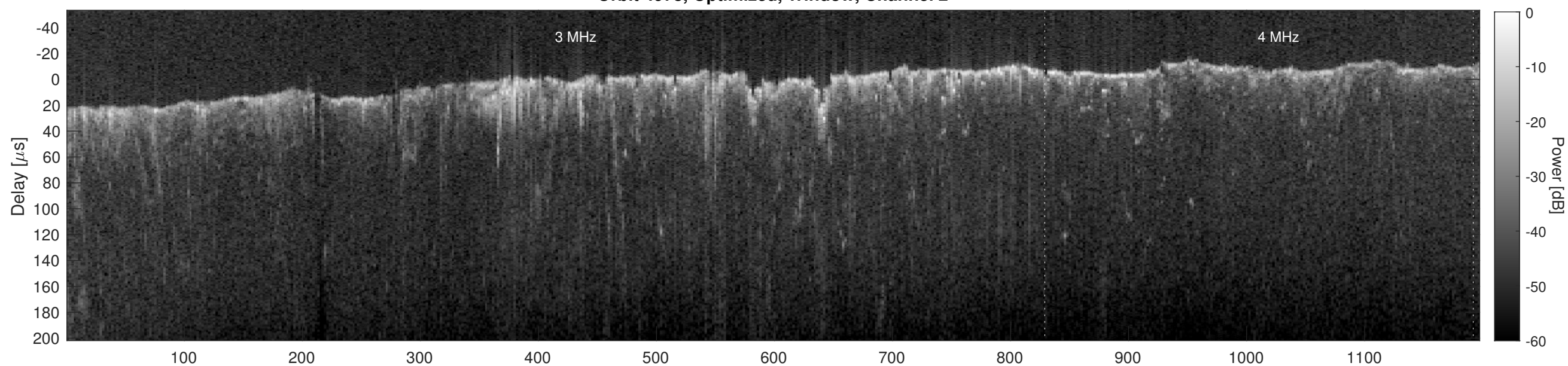
Orbit 4978, Cluttergram
