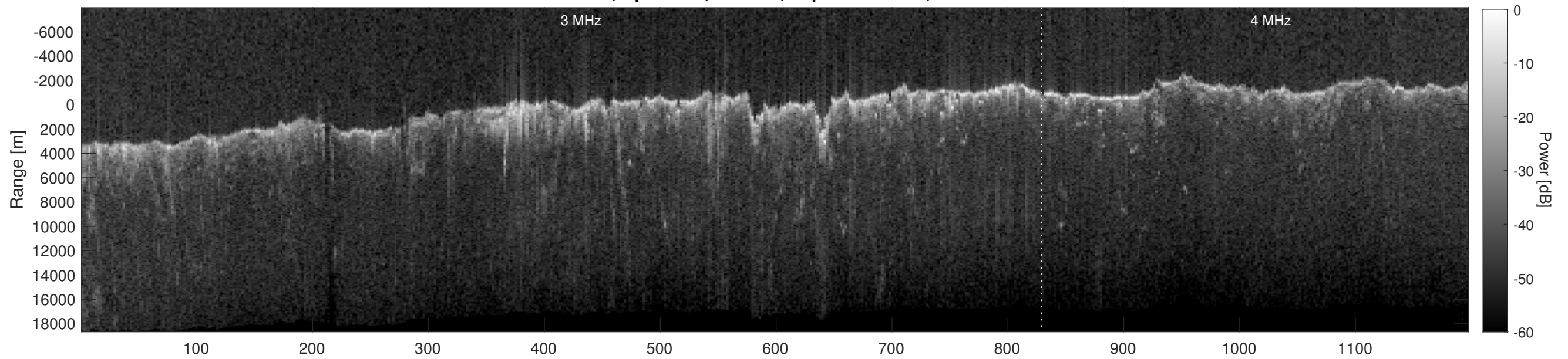
Orbit 4978, Depth-Corrected Cluttergram
