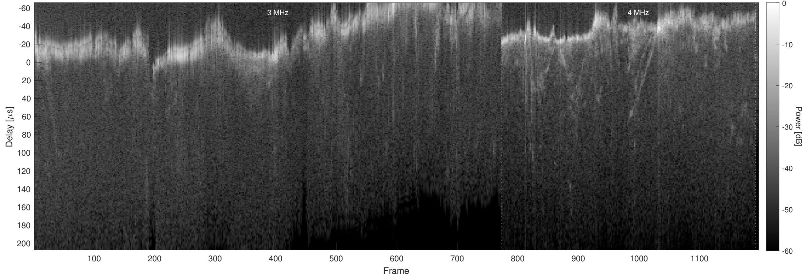
Orbit 4980, Chapman, No Window, Channel 2
