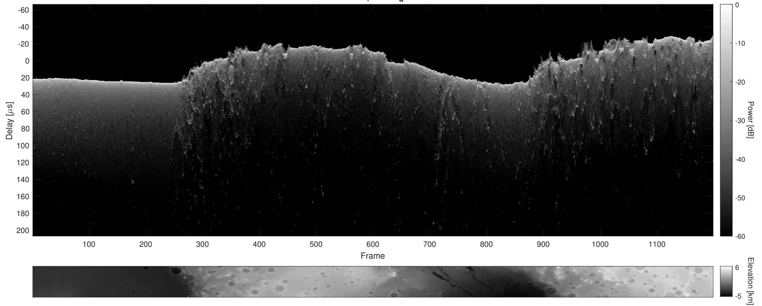
Orbit 4981, Cluttergram
