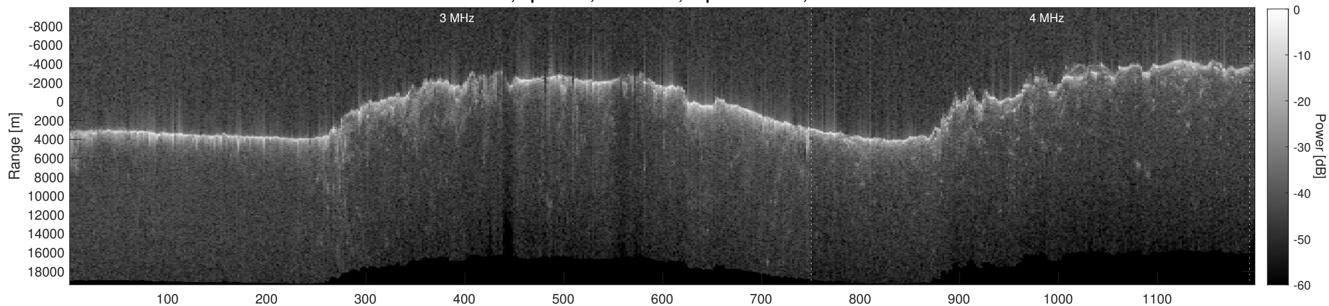
Orbit 4981, Depth-Corrected Cluttergram
