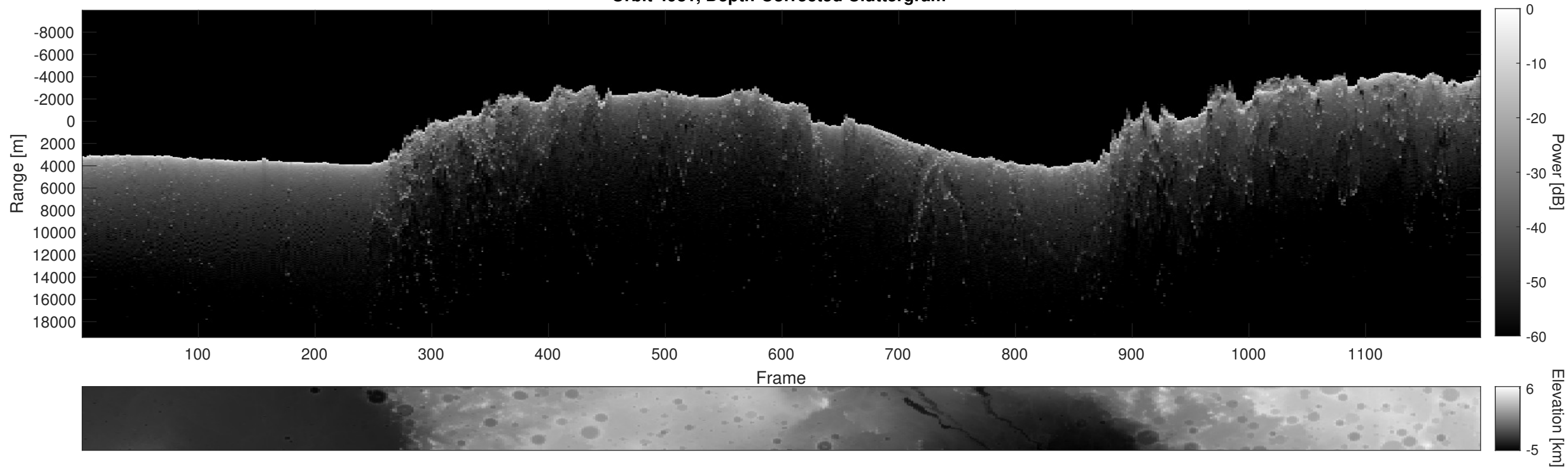
Orbit 4981, Depth-Corrected Cluttergram
