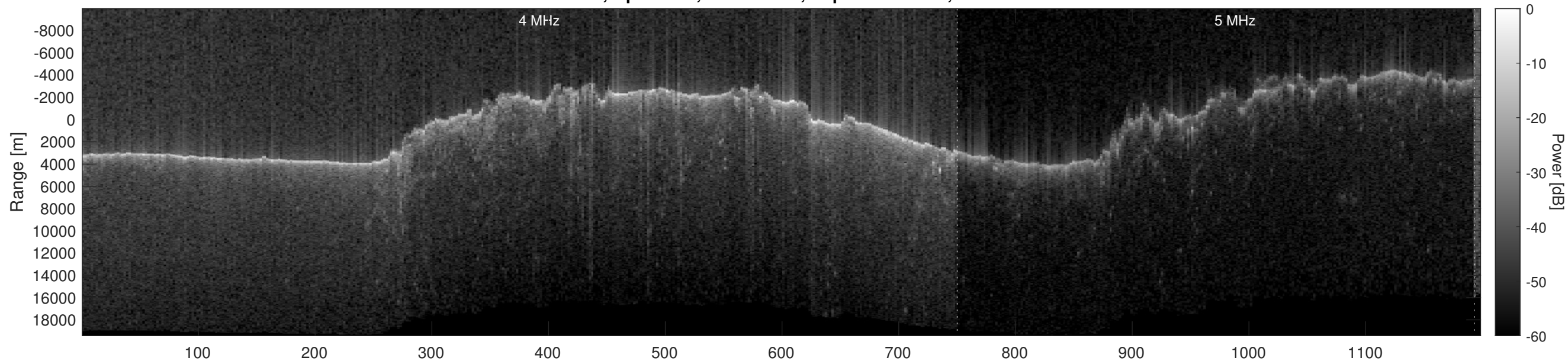
Orbit 4981, Optimized, No Window, Depth-Corrected, Channel 2
