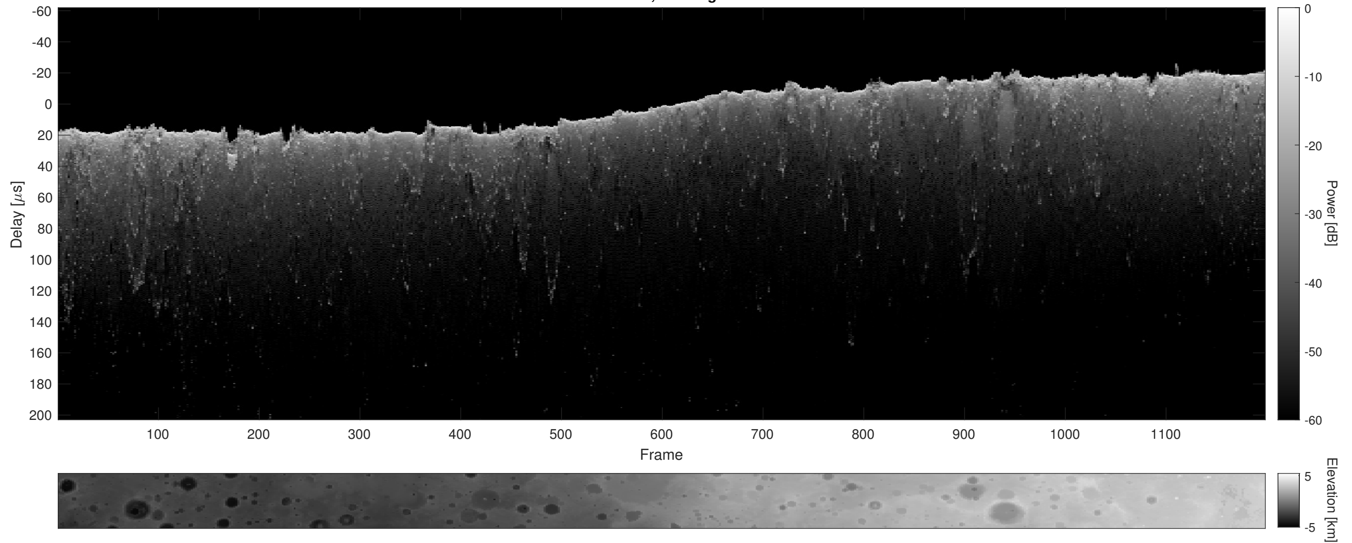
Orbit 4982, Cluttergram
