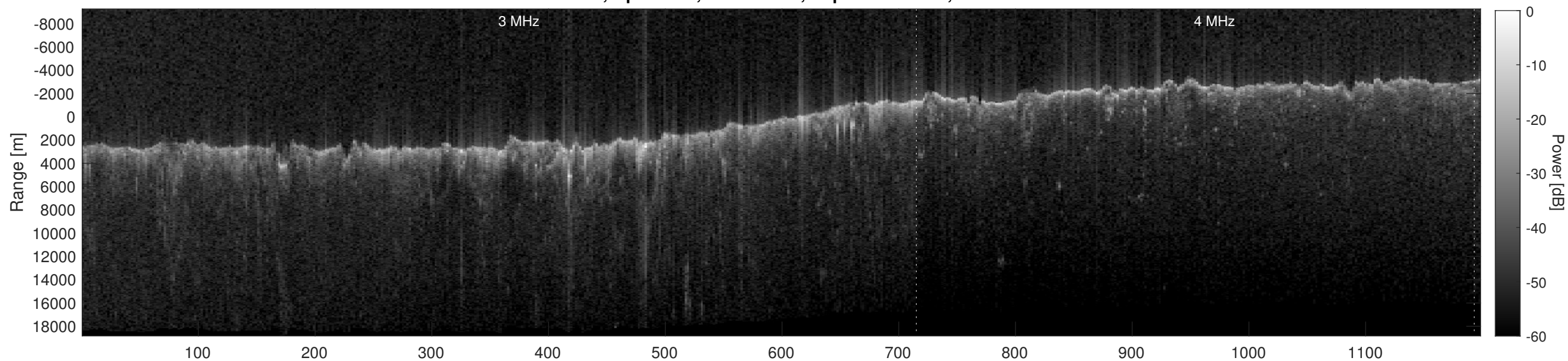
Orbit 4982, Depth-Corrected Cluttergram
