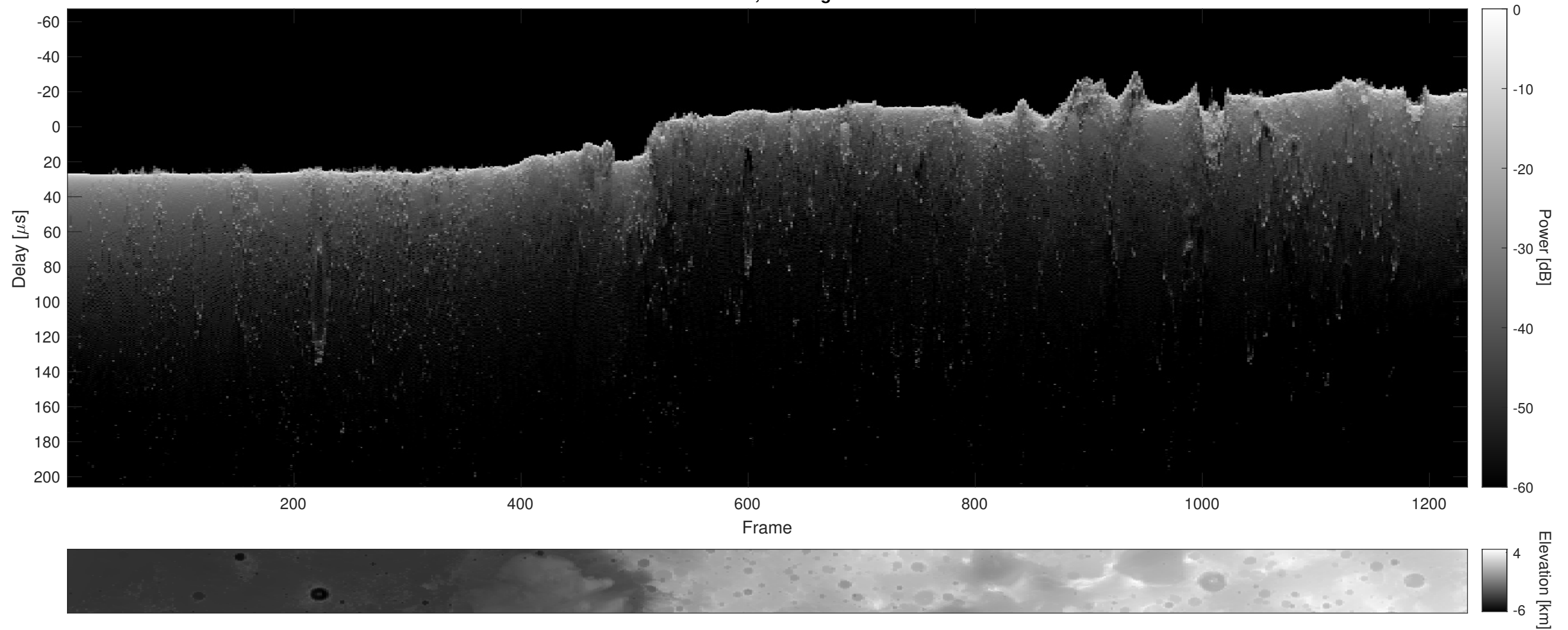
Orbit 4991, Cluttergram
