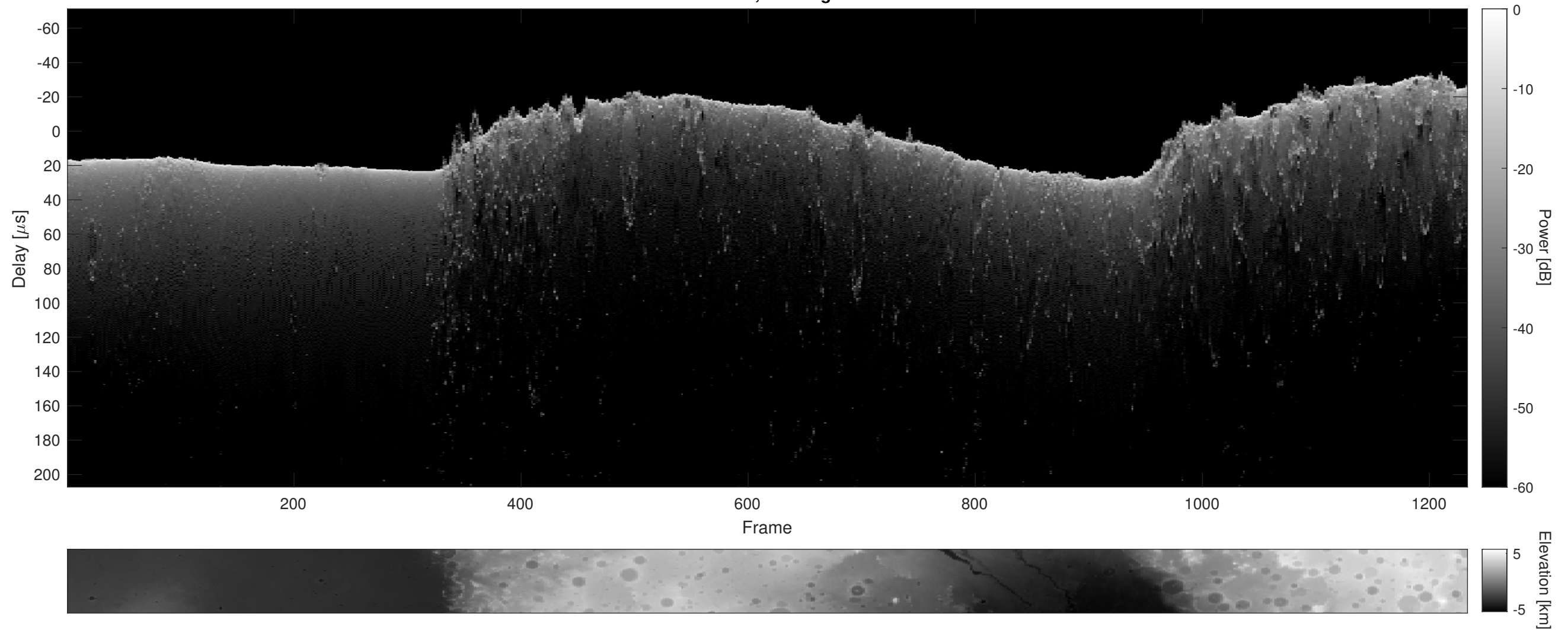
Orbit 4992, Cluttergram
