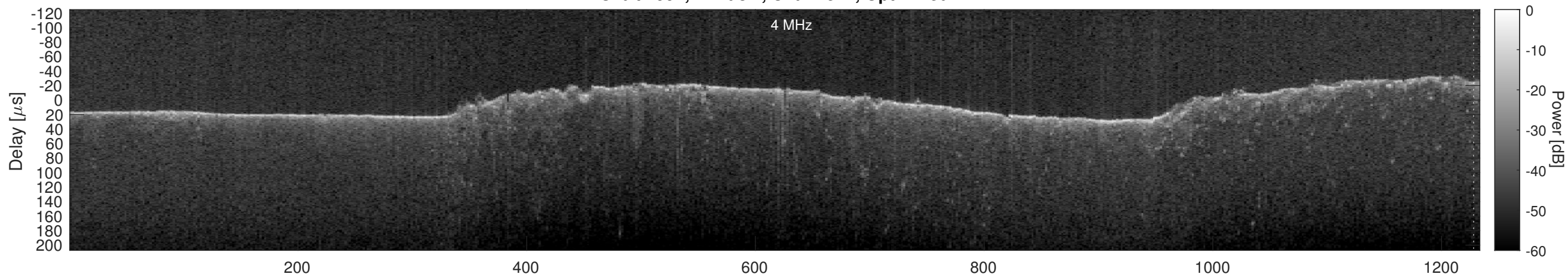
Orbit 4992, Cluttergram
