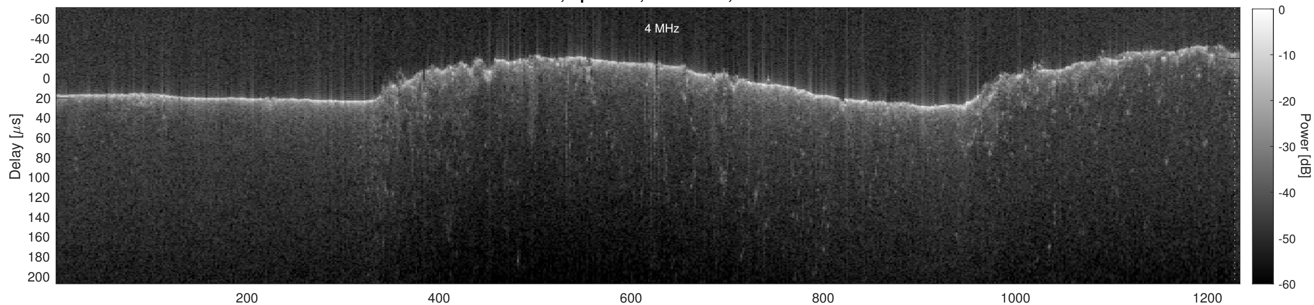
Orbit 4992, Cluttergram
