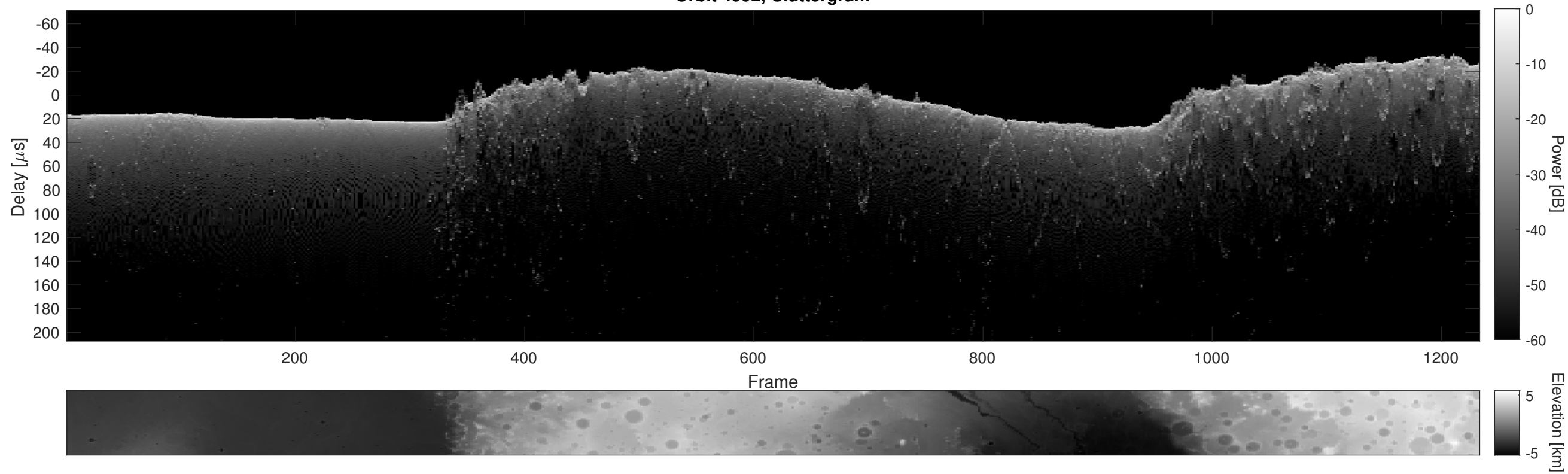
Orbit 4992, Cluttergram
