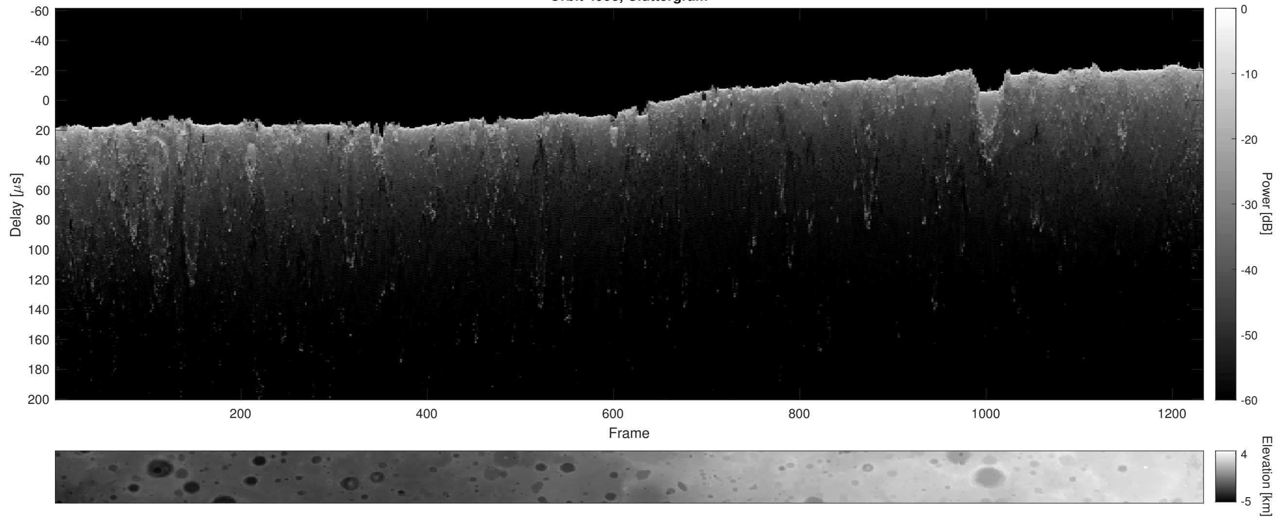
Orbit 4993, Cluttergram
