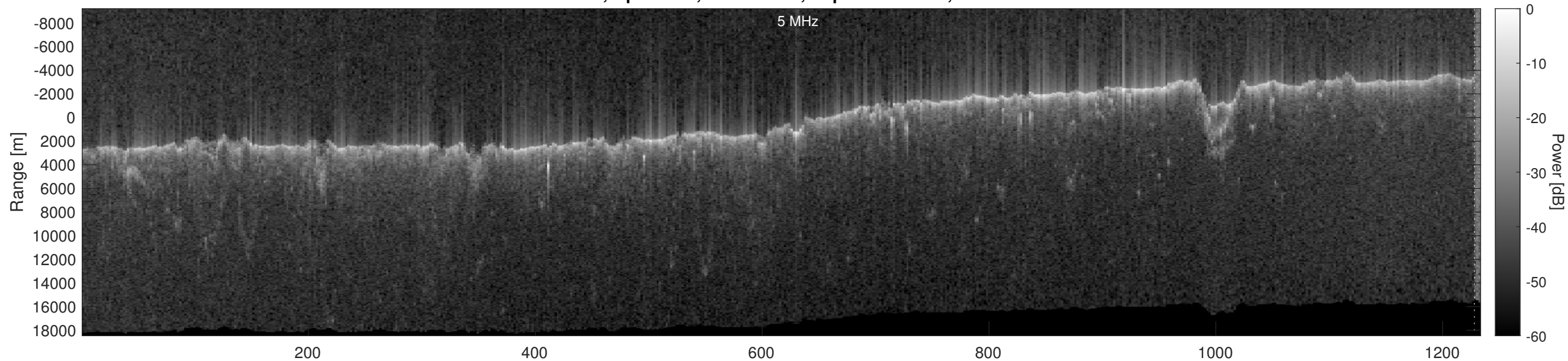
Orbit 4993, Optimized, No Window, Depth-Corrected, Channel 2
