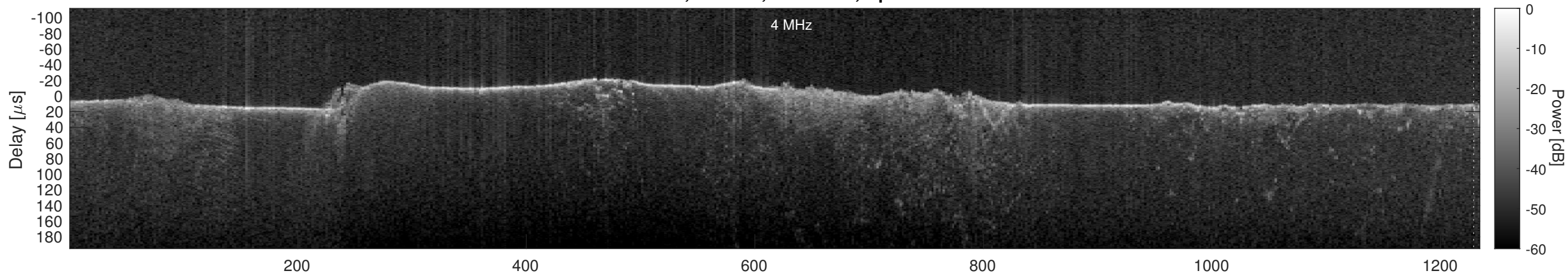
Orbit 4994, Cluttergram
