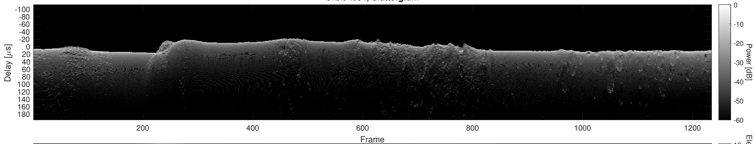
Orbit 4994, Cluttergram
