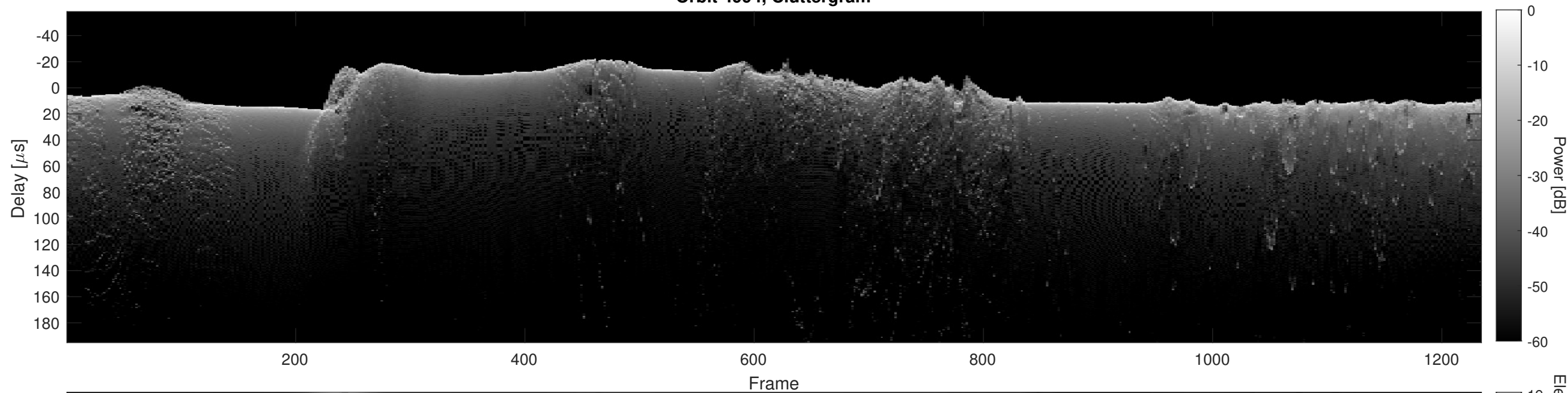
Orbit 4994, Cluttergram
