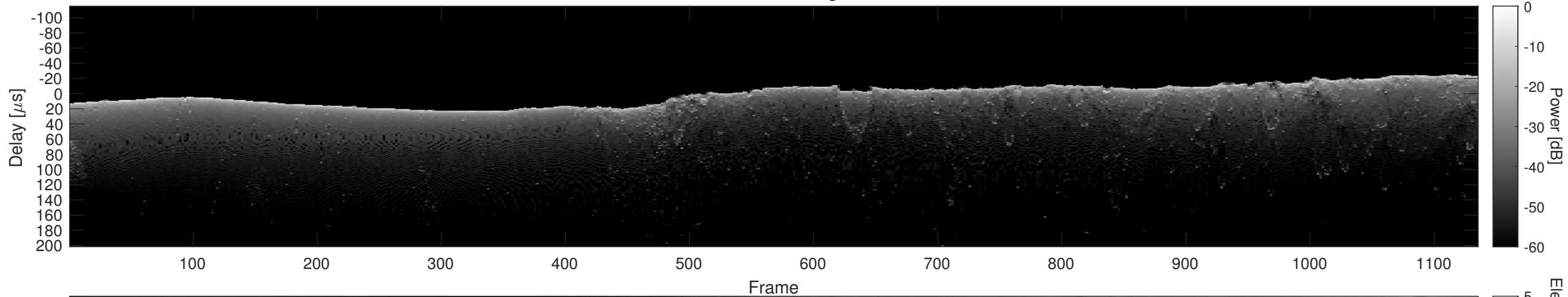
Orbit 4995, Cluttergram
