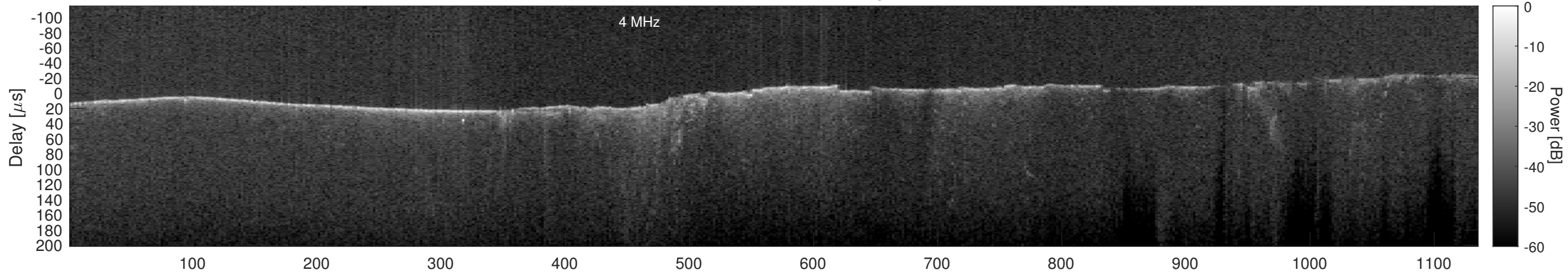
Orbit 4995, Cluttergram
