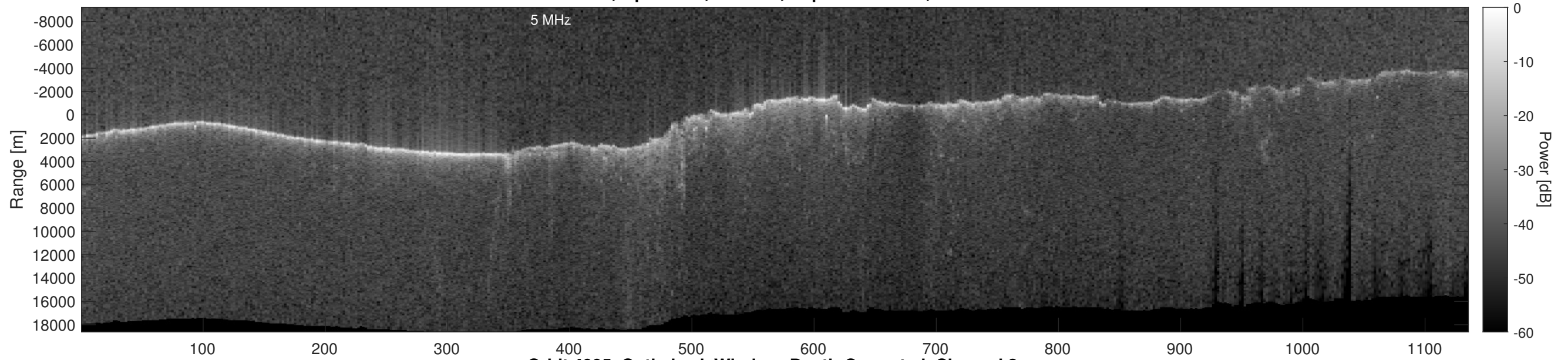
Orbit 4995, Optimized, Window, Depth-Corrected, Channel 2
