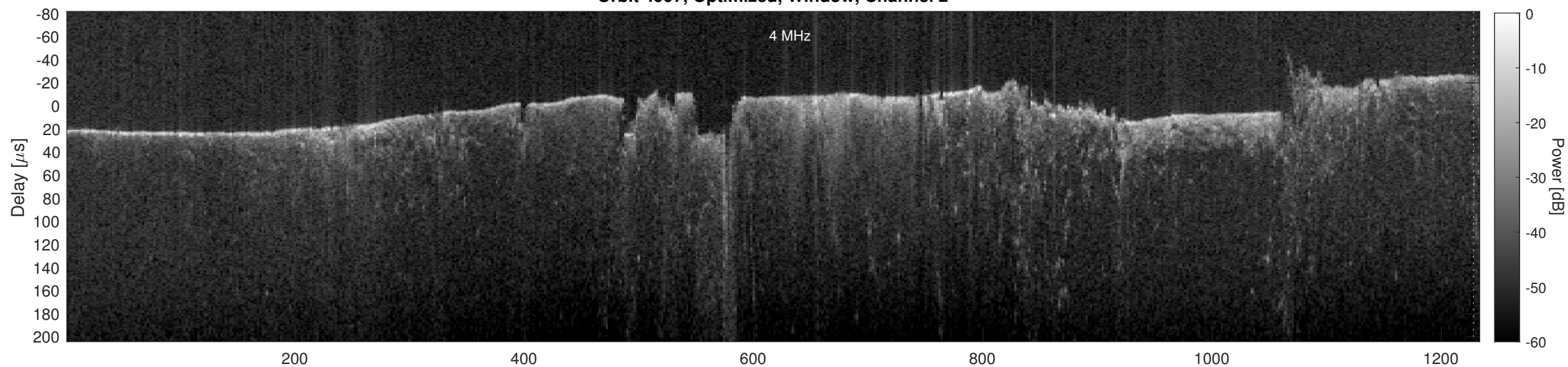
Orbit 4997, Cluttergram
