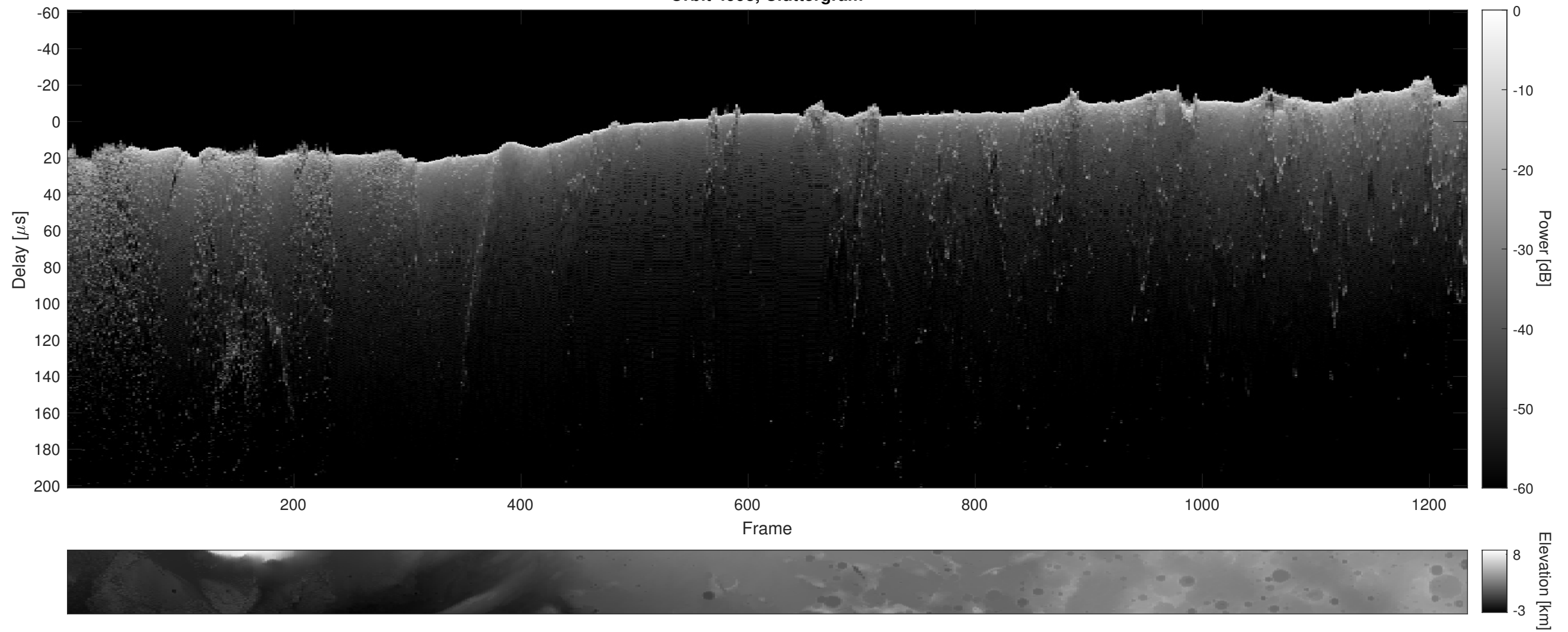
Orbit 4998, Cluttergram
