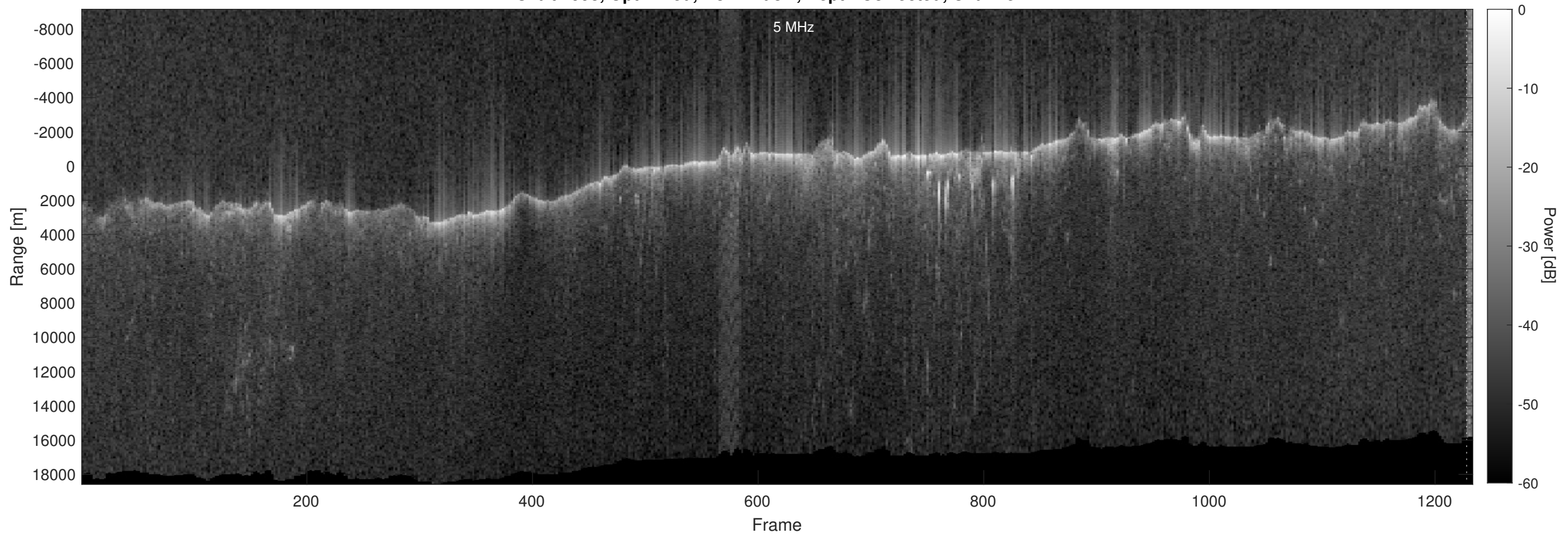
Orbit 4998, Optimized, No Window, Depth-Corrected, Channel 2
