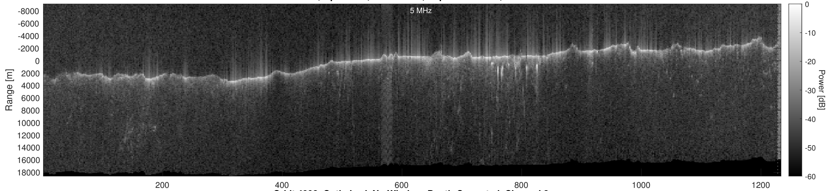
Orbit 4998, Optimized, No Window, Depth-Corrected, Channel 2
