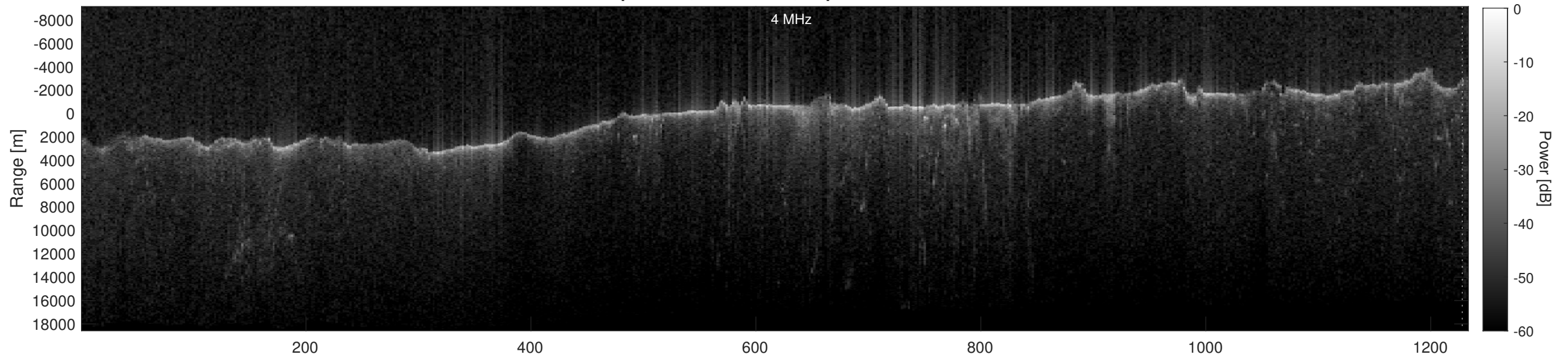
Orbit 4998, Depth-Corrected Cluttergram
