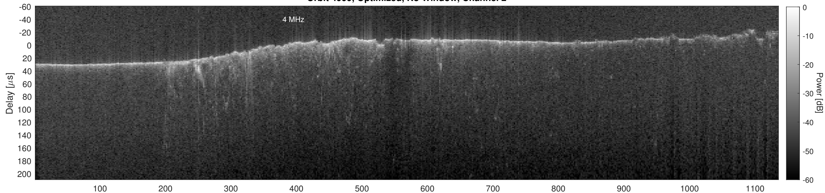
Orbit 4999, Cluttergram
