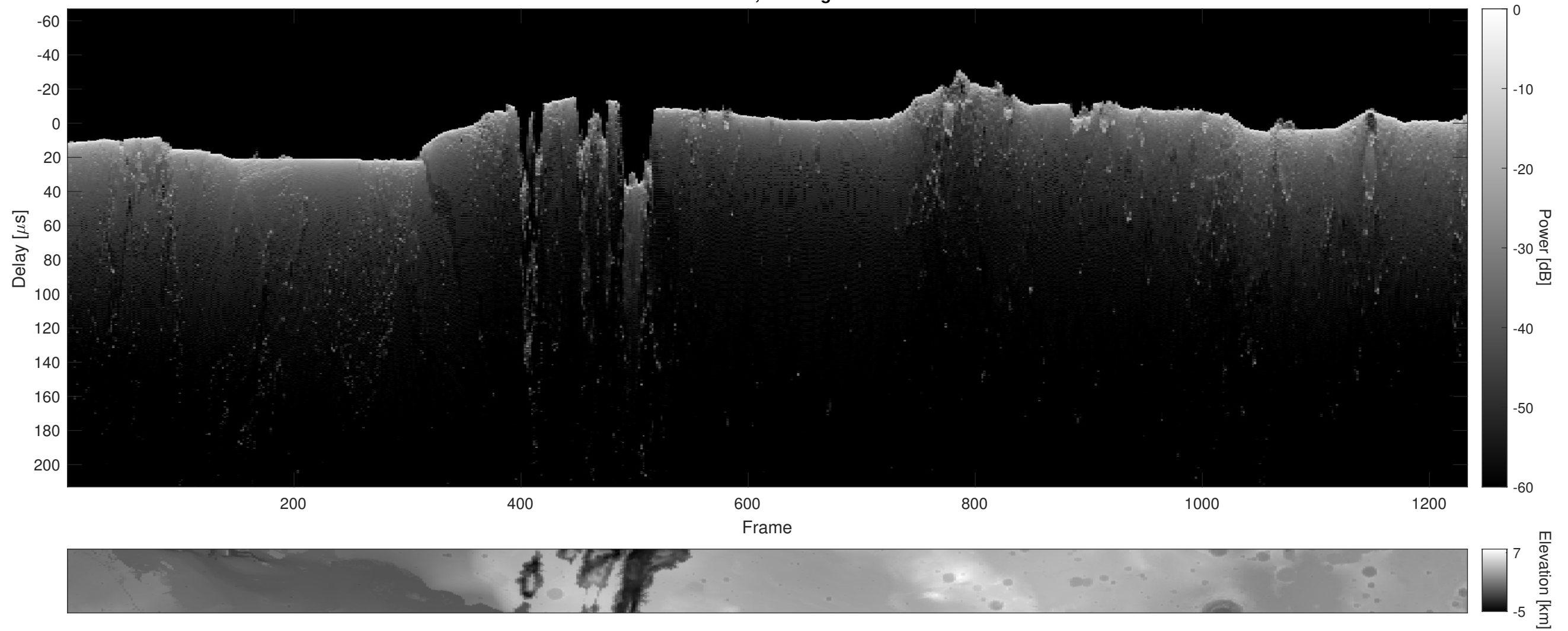
Orbit 5001, Cluttergram
