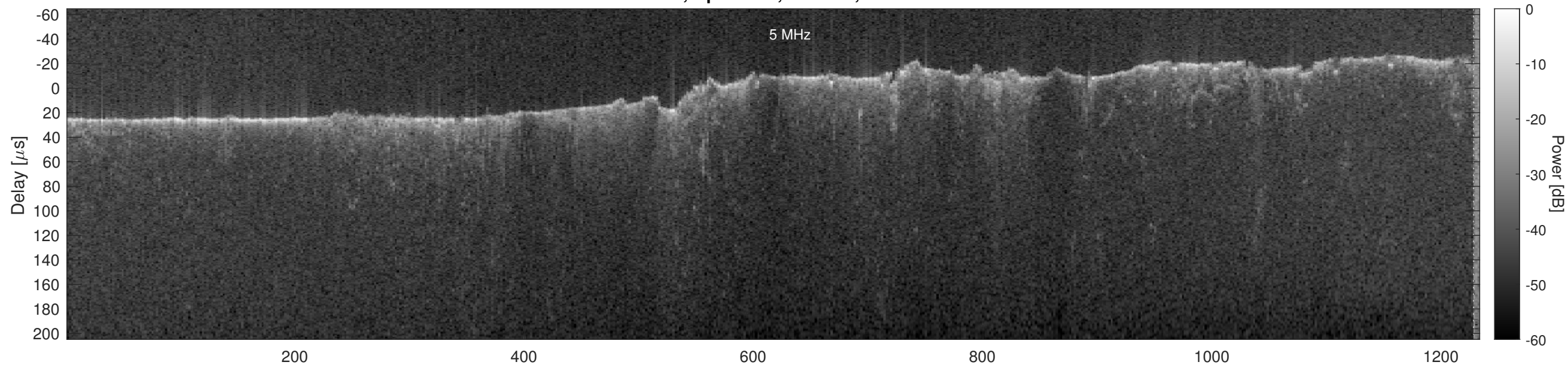
Orbit 5002, Optimized, Window, Channel 2
