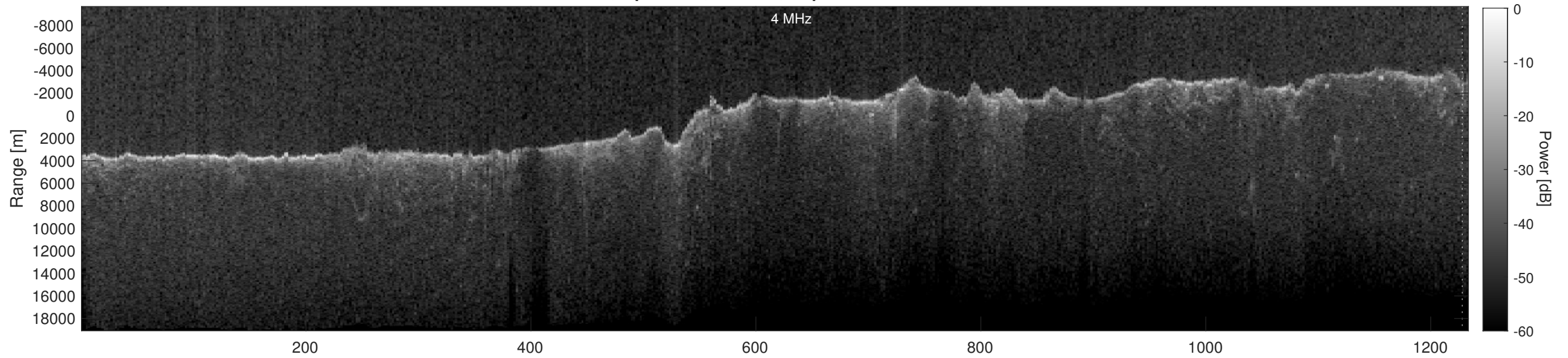
Orbit 5002, Depth-Corrected Cluttergram
