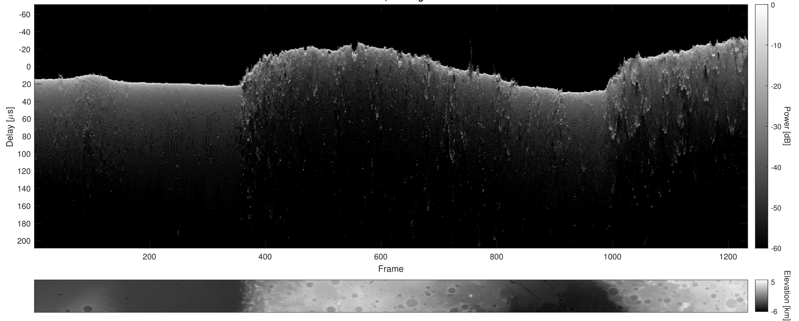
Orbit 5003, Cluttergram
