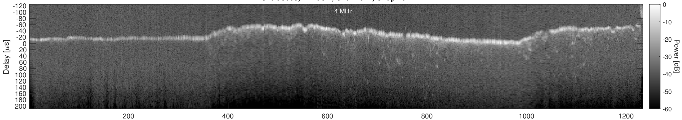
Orbit 5003, Window, Channel 2, Optimized
