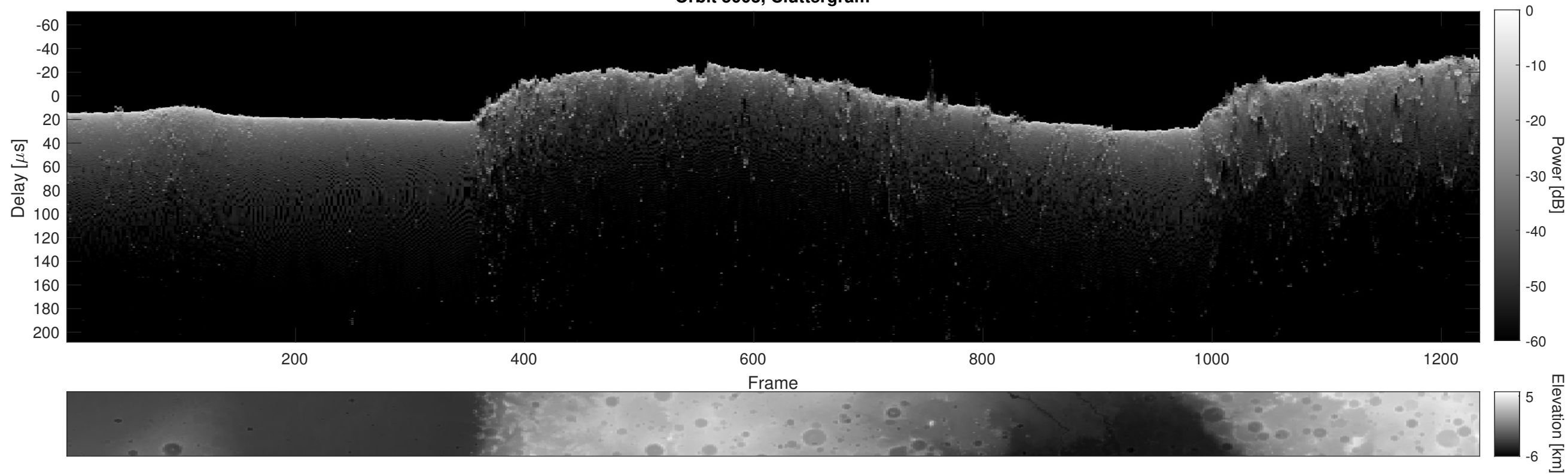
Orbit 5003, Cluttergram
