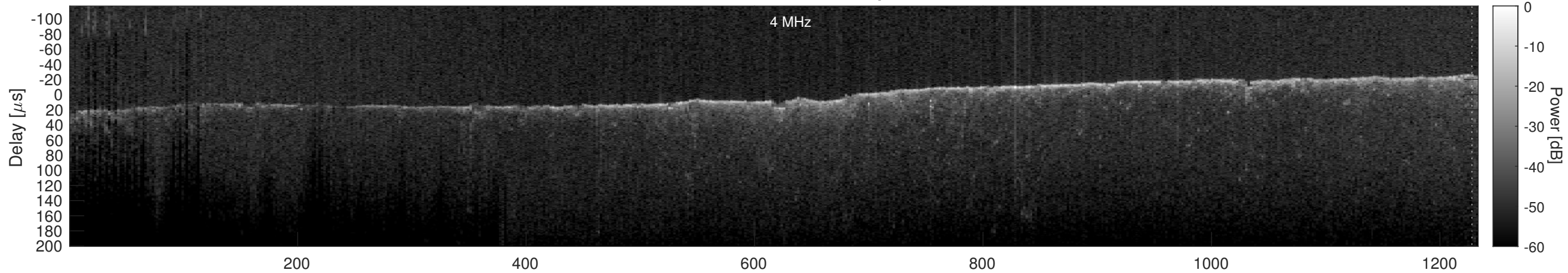
Orbit 5004, Cluttergram
