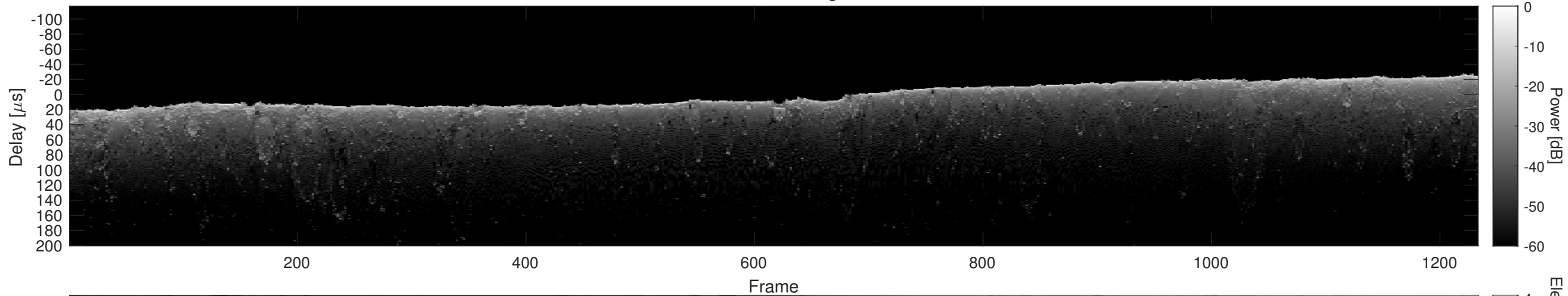
Orbit 5004, Cluttergram
