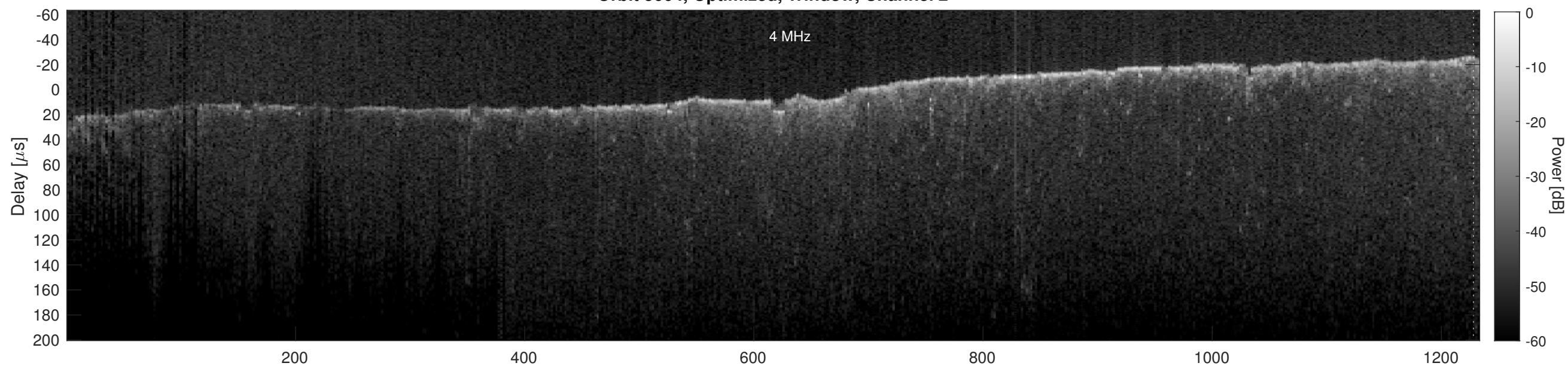
Orbit 5004, Cluttergram
