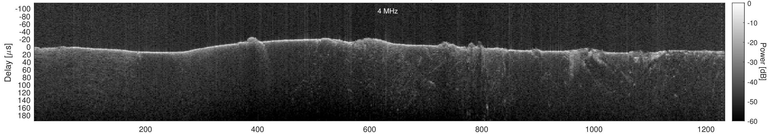
Orbit 5005, Cluttergram
