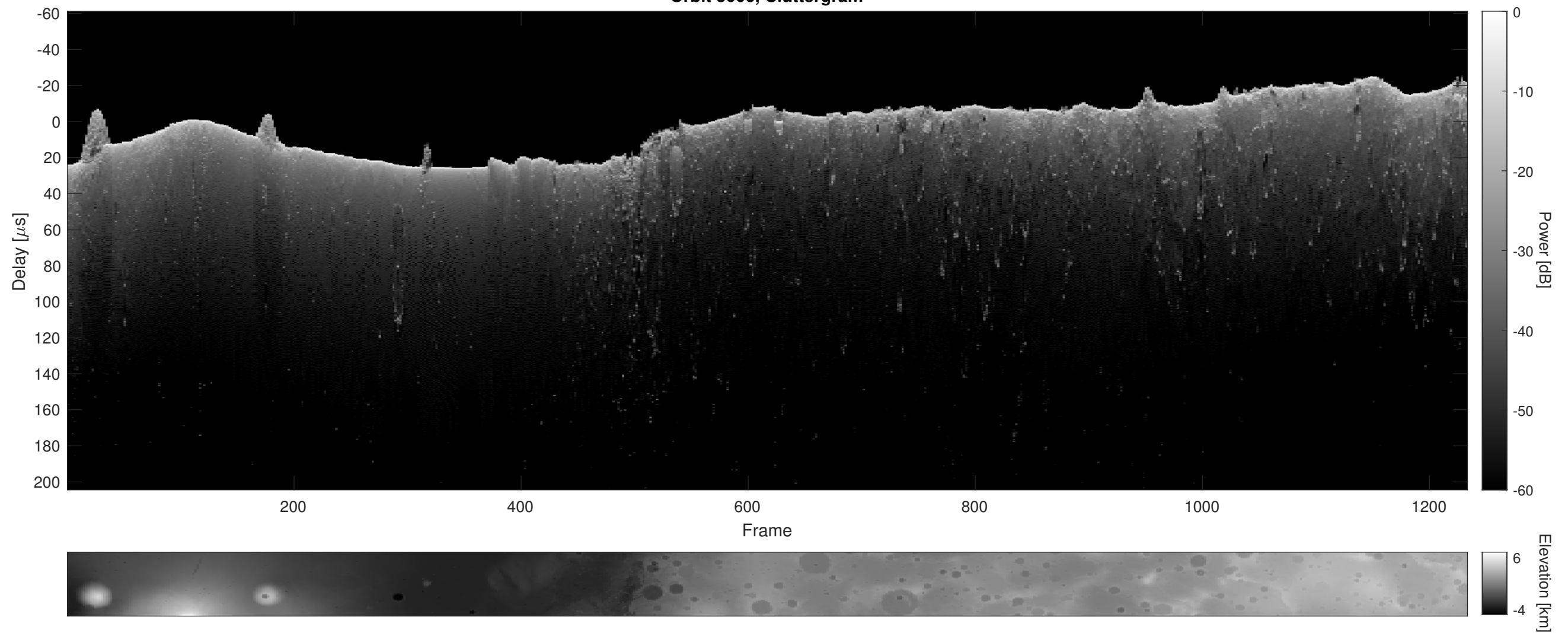
Orbit 5006, Cluttergram
