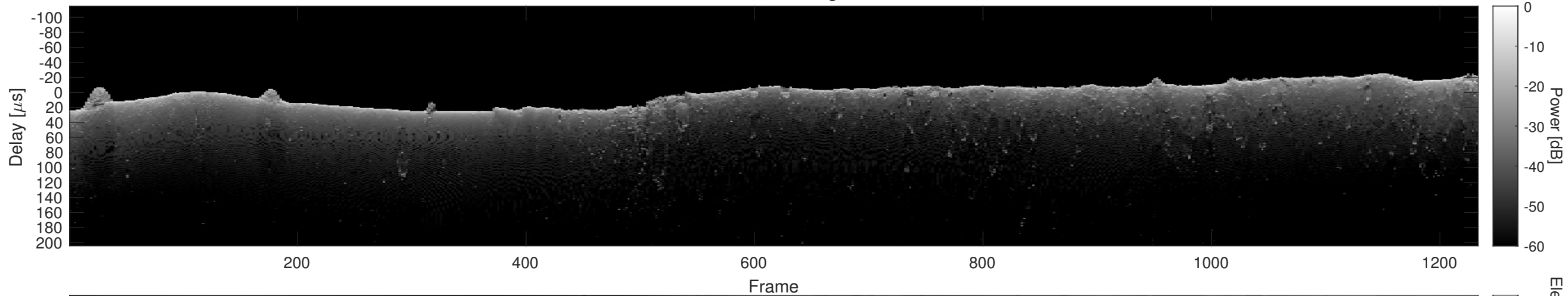
Orbit 5006, Cluttergram
