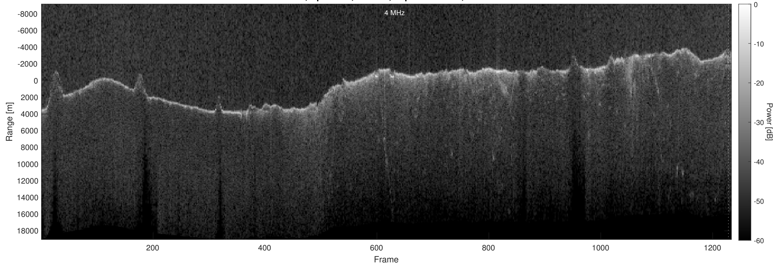
Orbit 5006, Optimized, Window, Depth-Corrected, Channel 2
