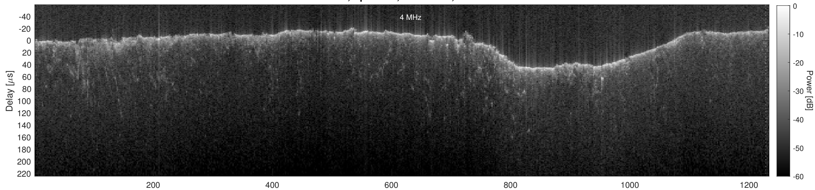
Orbit 5007, Cluttergram
