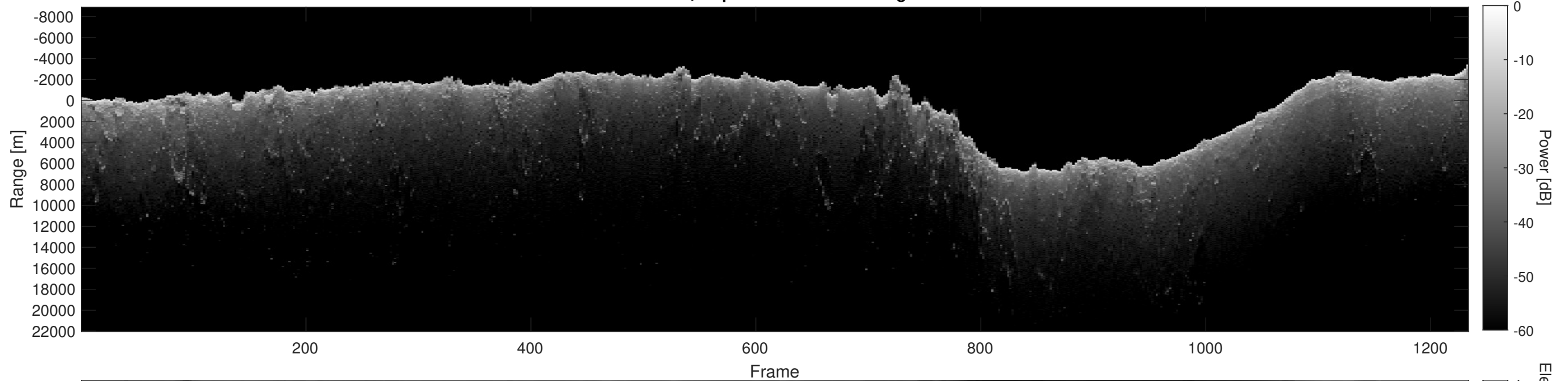
Orbit 5007, Depth-Corrected Cluttergram
