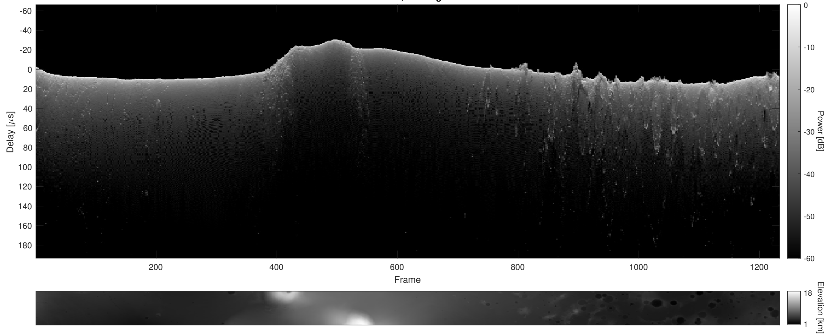
Orbit 5016, Cluttergram
