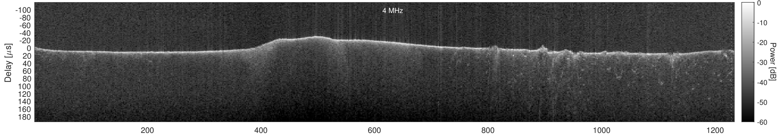
Orbit 5016, Cluttergram
