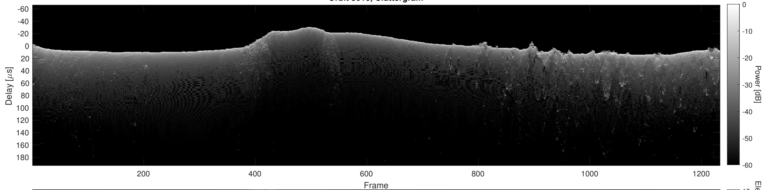
Orbit 5016, Cluttergram
