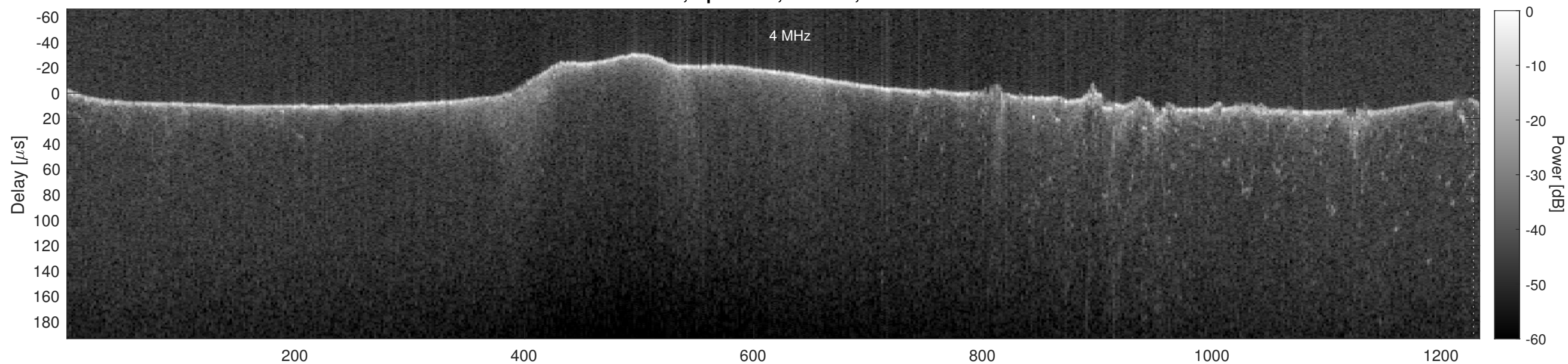
Orbit 5016, Cluttergram
