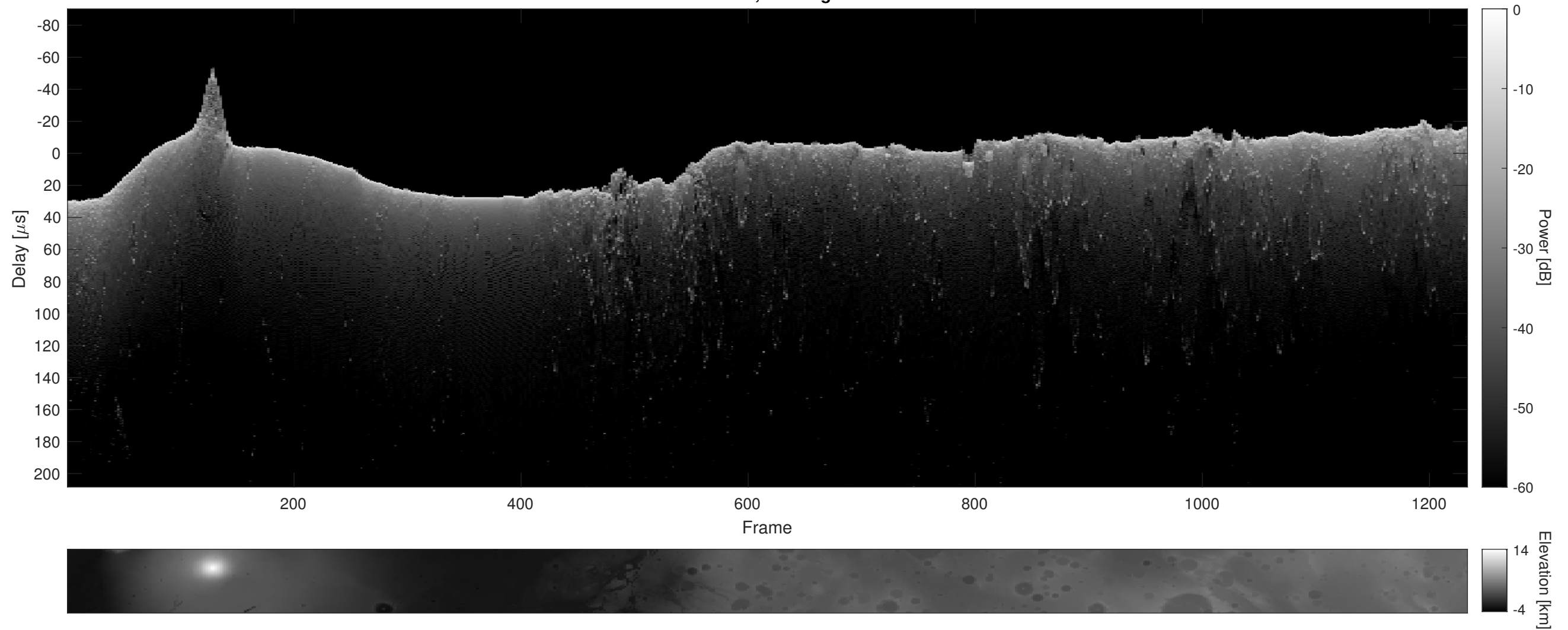
Orbit 5017, Cluttergram
