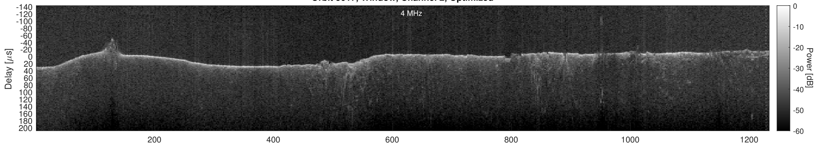
Orbit 5017, Cluttergram
