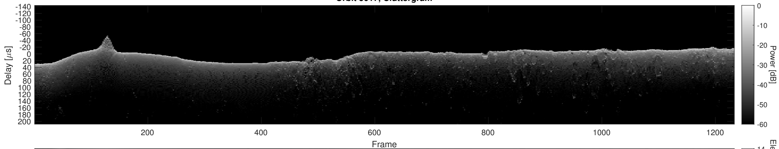
Orbit 5017, Cluttergram
