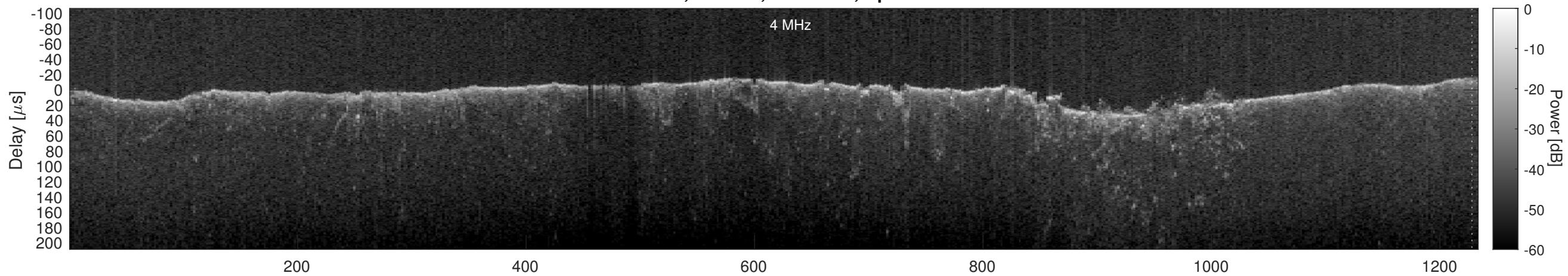
Orbit 5018, Cluttergram
