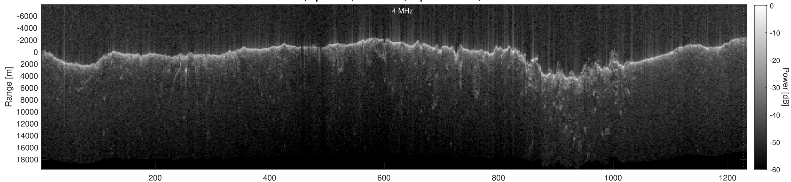
Orbit 5018, Depth-Corrected Cluttergram
