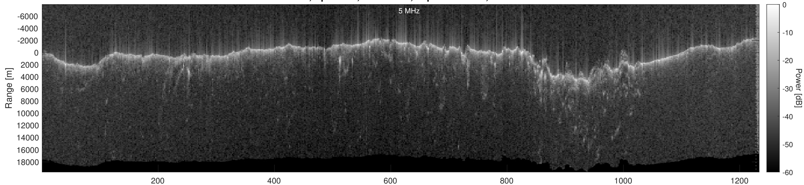
Orbit 5018, Optimized, No Window, Depth-Corrected, Channel 2
